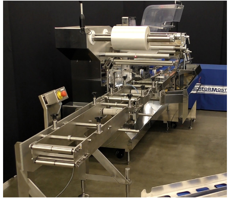
ATTACHLESS INFEED WITHOUT BELTS
