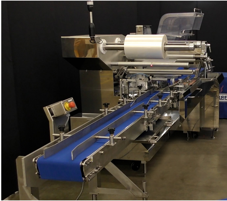
ATTACHLESS INFEED WITH BELTS
